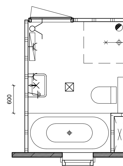
badkamerindeling 1 - ligbad
